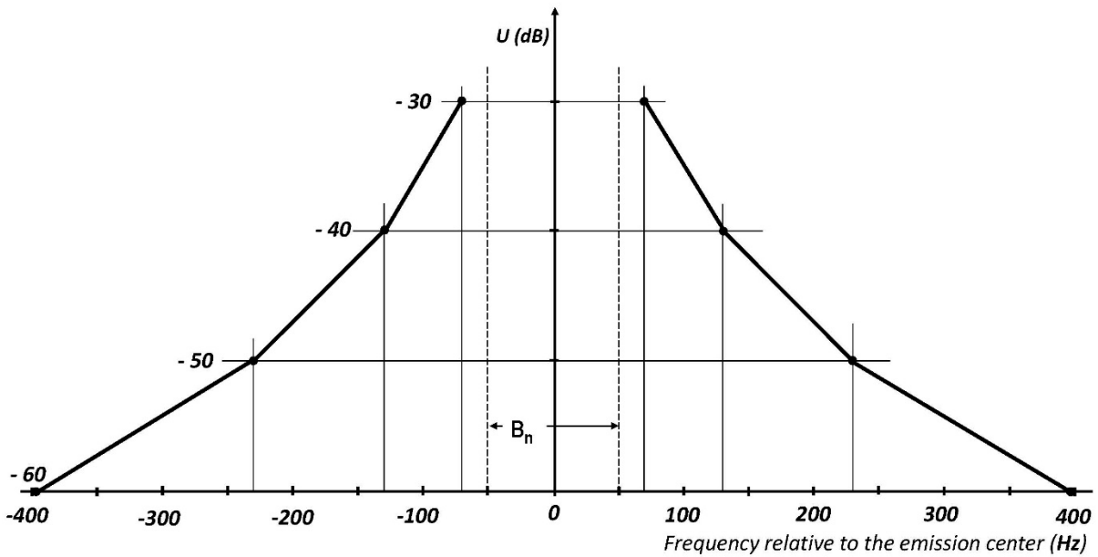
FIGURE 1 OoB emission masks for classes of emissions G1B and G1D
