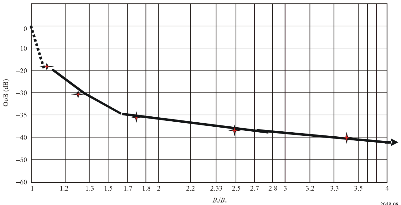
Comparing OoB measurements with specified limits for class J3EJN (transmitter of the fixed service)
